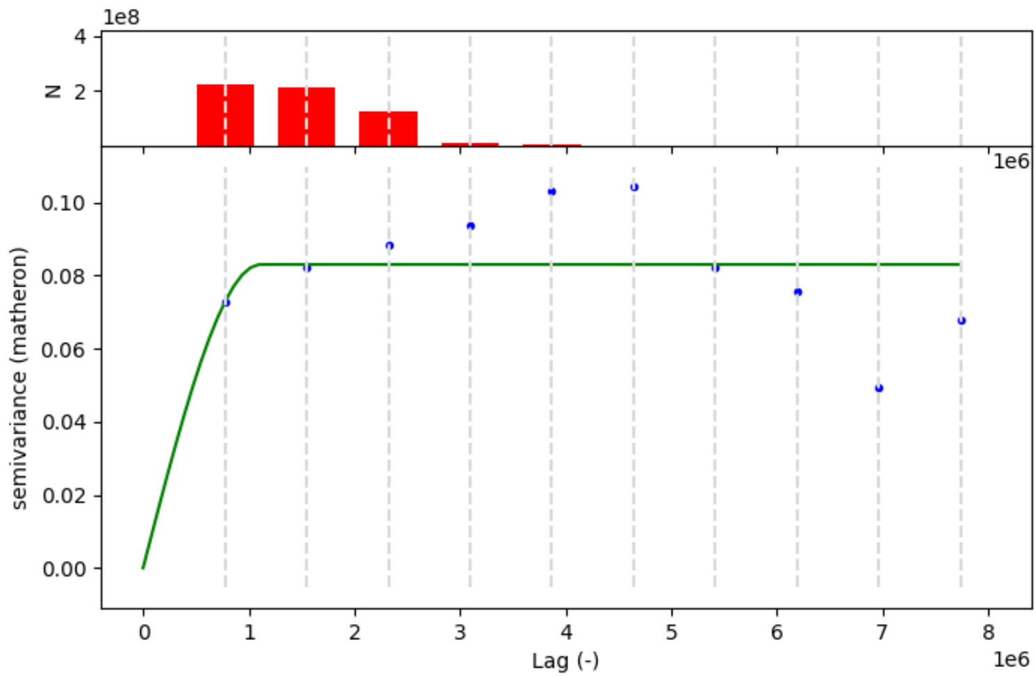
Figure XXX. Semivariogram of prediction probability and actual target classification. Lag is in m^2
