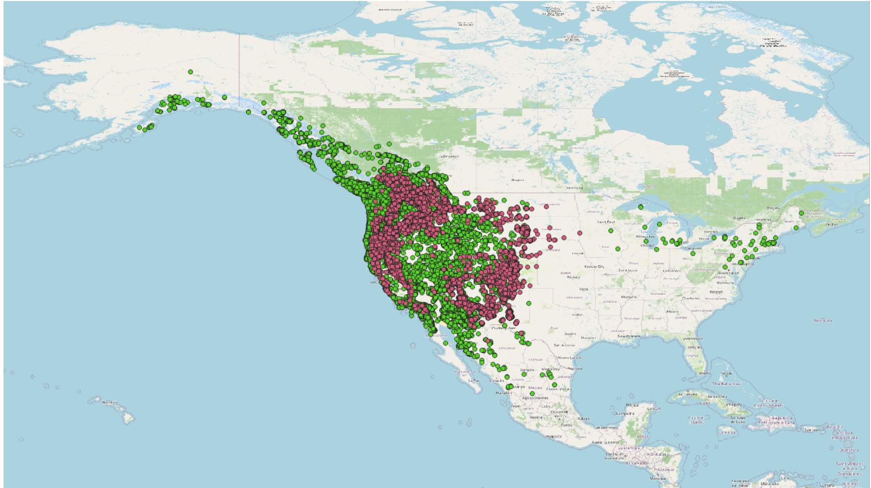
Figure S1. Presence and absence points from GBIF used in the predictive model. Red is presence, green is absence
